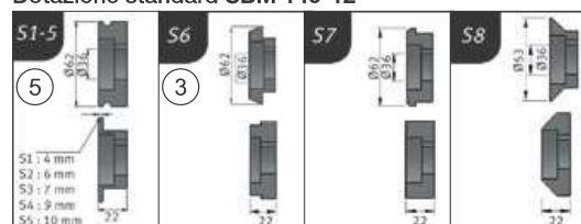
S1-5: Rulli standard per Ø 4/6/7/9/10 mm
